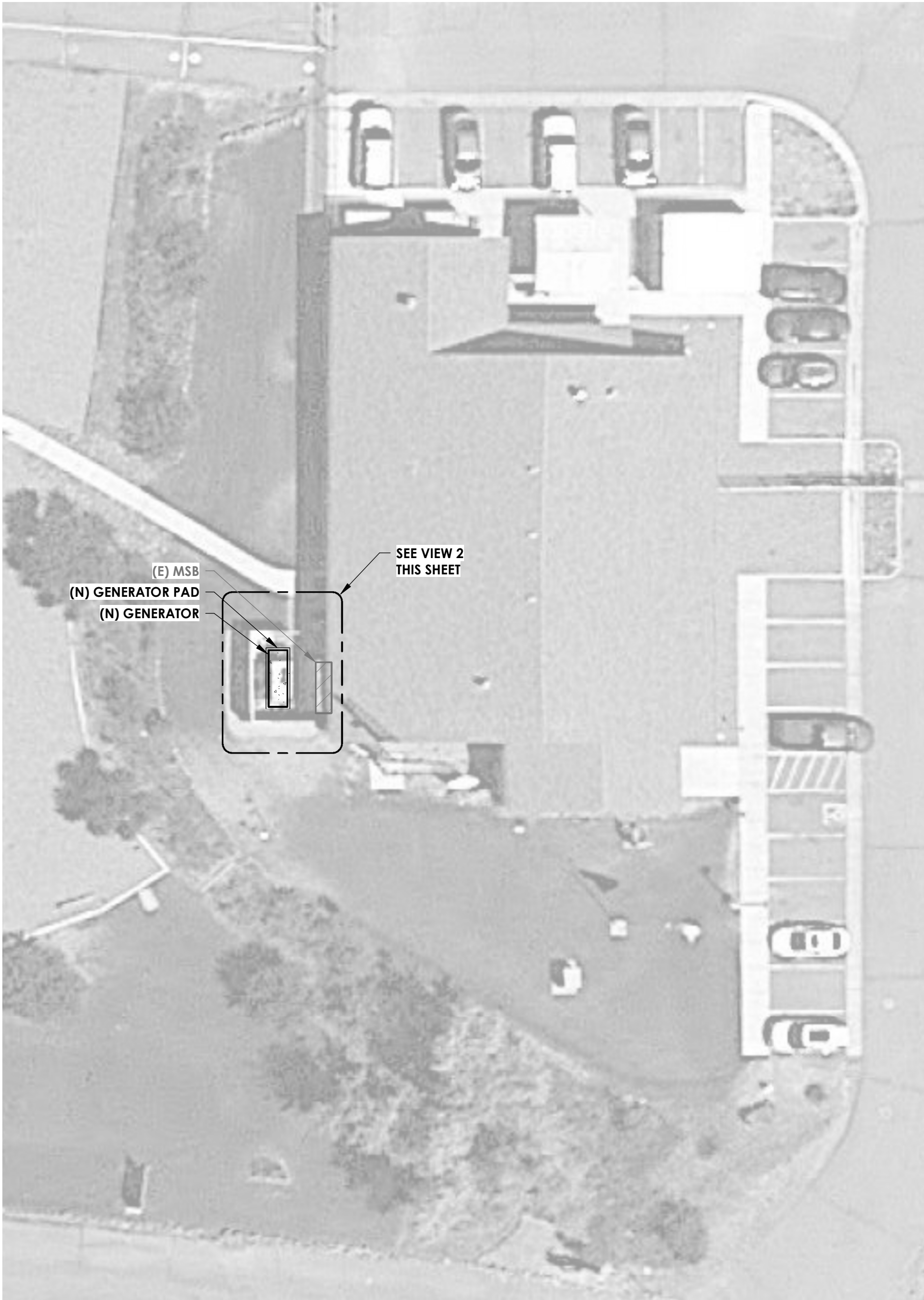
PLUMBING SITE PLAN 1 1" = 20'-0" P1
