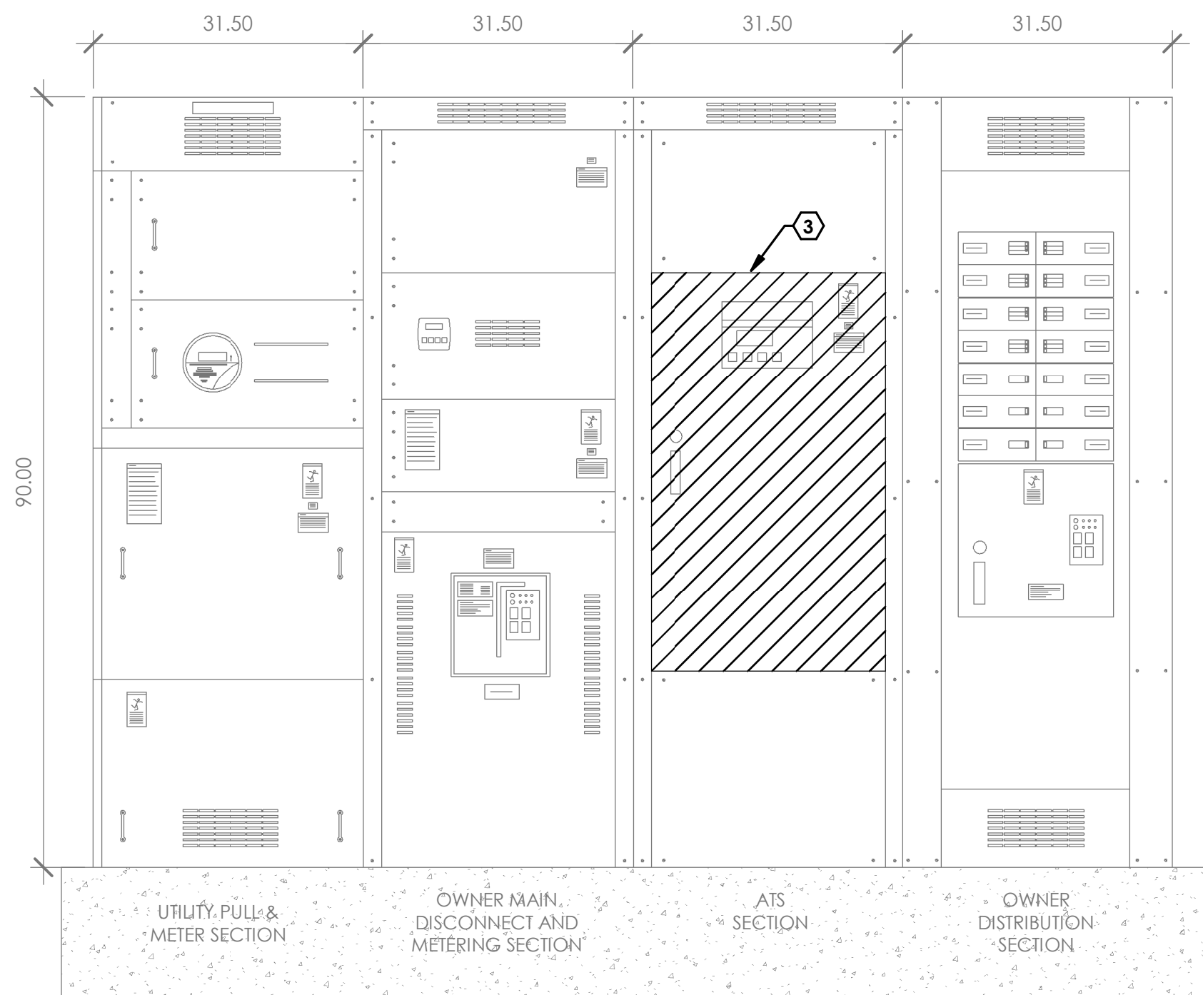
EXISTING MSB ELEVATION - DEMO 3/4" = 1'-0" 1 E3
