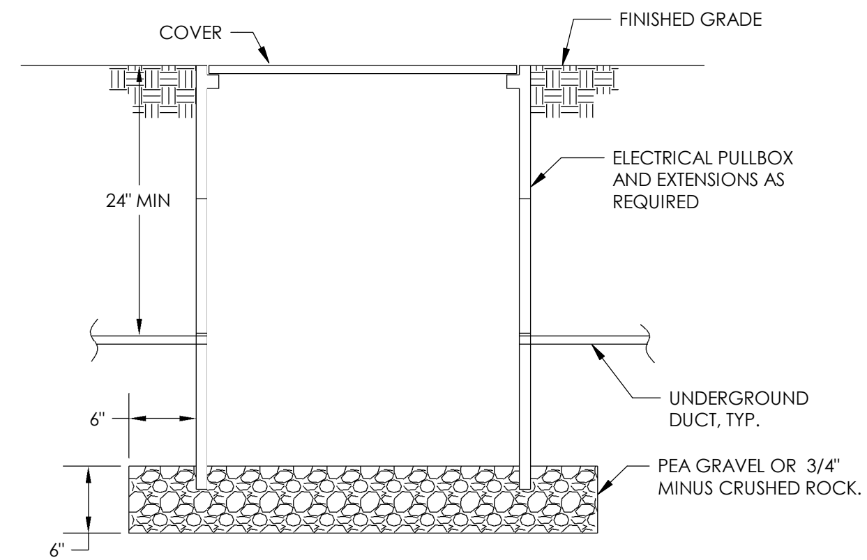
PULLBOX - PULL THROUGH NTS 5 E3
