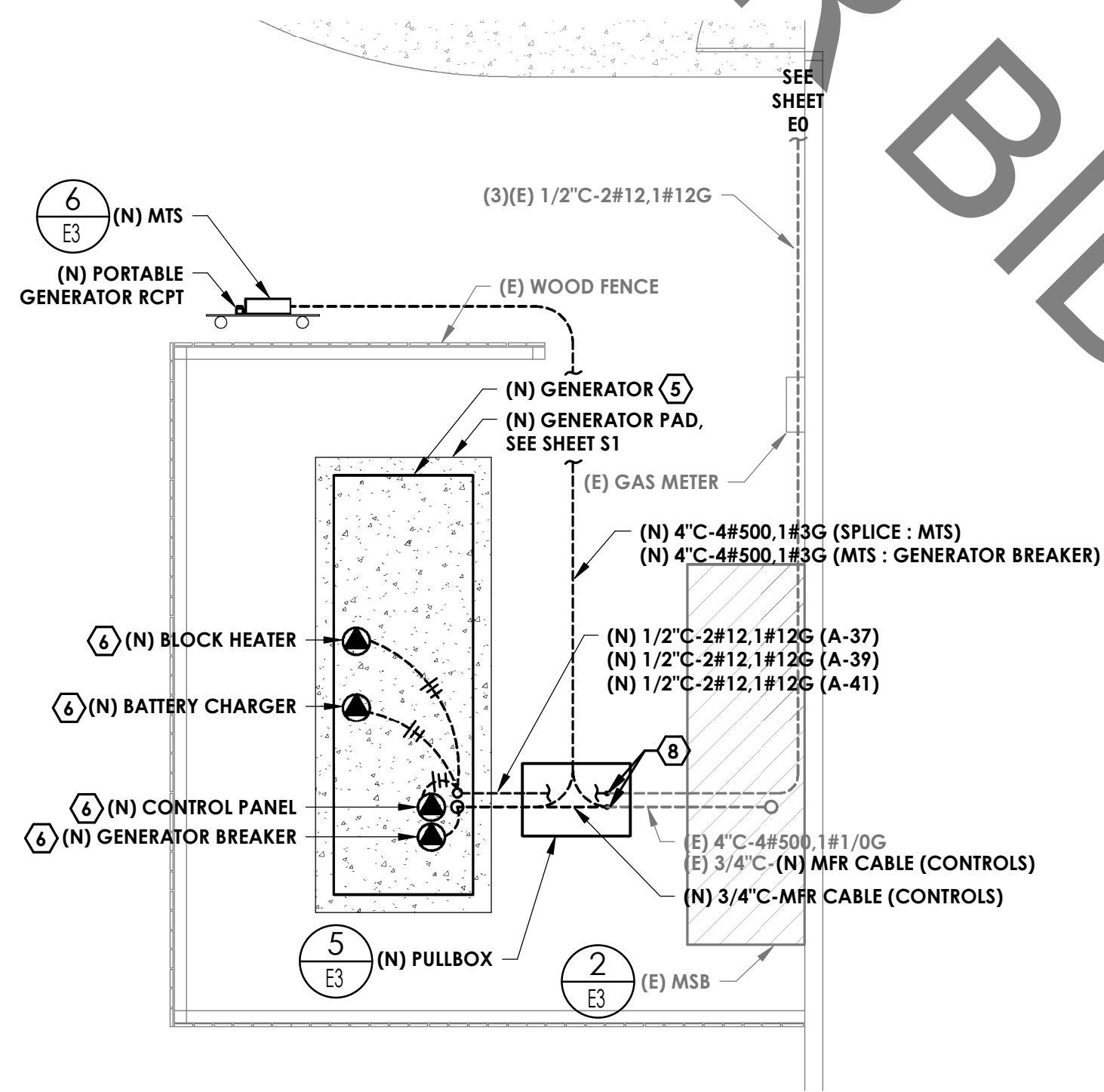
GENERATOR POWER PLAN - NEW 1/4" = 1'-0" 4 E3
