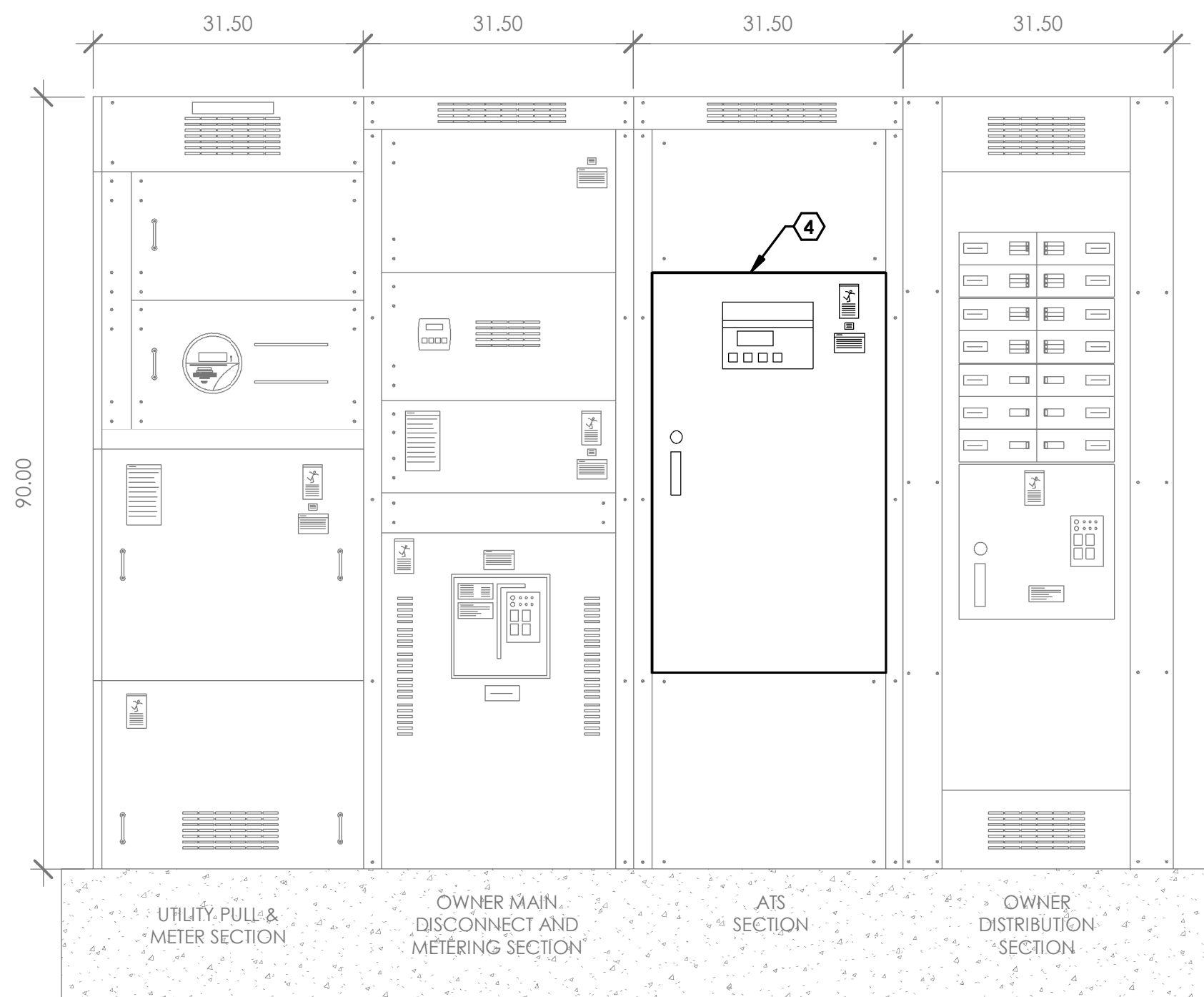
EXISTING MSB ELEVATION - NEW 3/4" = 1'-0" 2 E3
